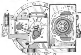
Figs. 2513-2514. Side View.
